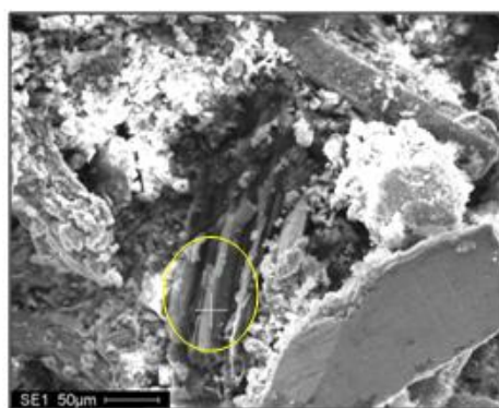
Figure 4.16 Carbon fibers identification
