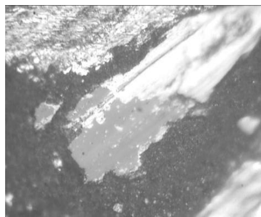
4.14b Adhesive wear – Pad
