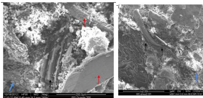
Figure 4.15 SEM images have shown that clear picture about the distribution of fibers, metal particles and other particles.
