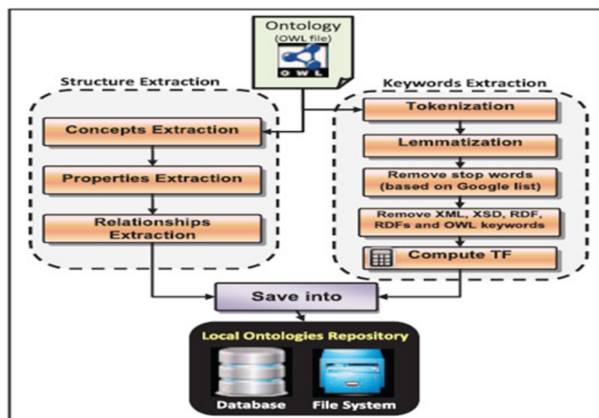
Figure 4.2 Local Ontology Repository
