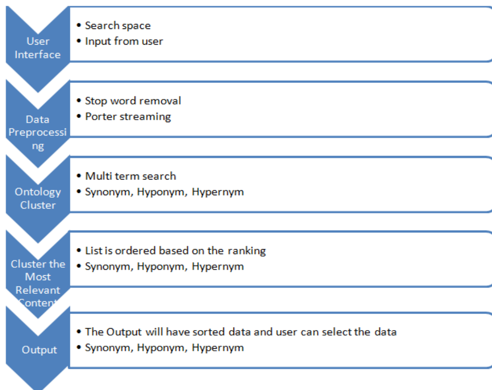
Figure 4.3 Ontology Web Crawler
