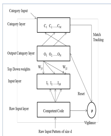
Figure 5: Architecture of Fuzzy ART Network
