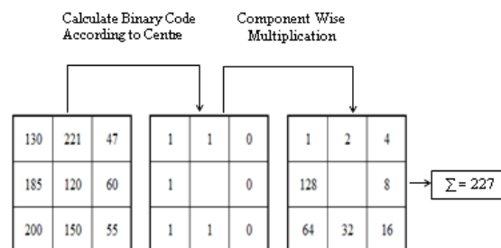
Figure 4: LBP Pattern Extraction Algorithm
