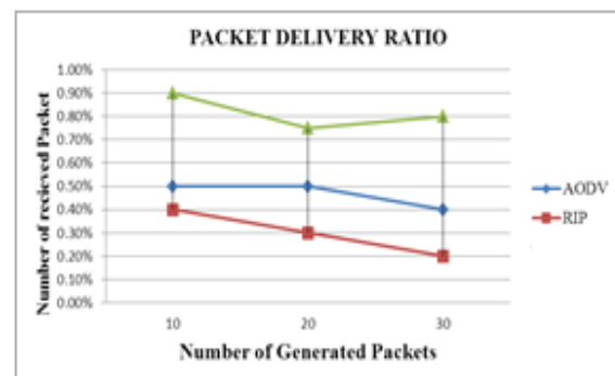
Figure 3. Graph Packet delivery ratio
