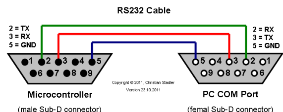
Figure 2. RS232
