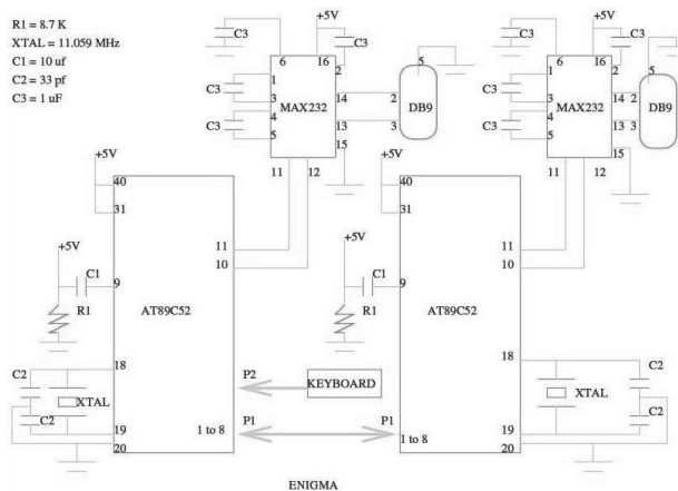
Figure 4. ENIGMA – Encryption/Decryption Module
