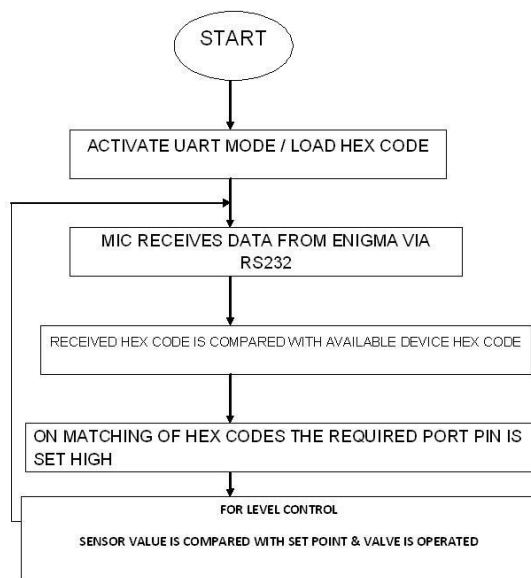
Figure 9. Local Controller Flow Diagram
