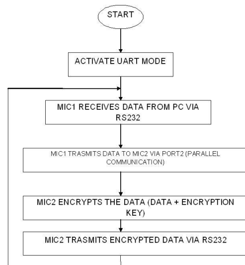
Figure 7. Encryption Flow Diagram
