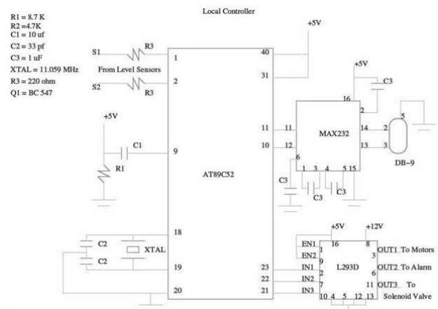
Figure 3. Local Controller
