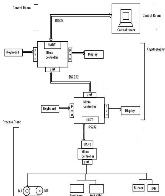
Figure 2. Simulation of Thermal Power Plant
