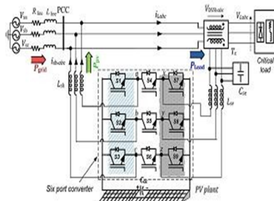
Fig. 2. Proposed integrated PV and DVR system configuration.
