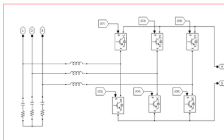
Fig (4) Second level of Proposed Dynamic voltage restorer
