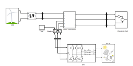
Fig 3 Simulation model of proposed dvr based solar system
