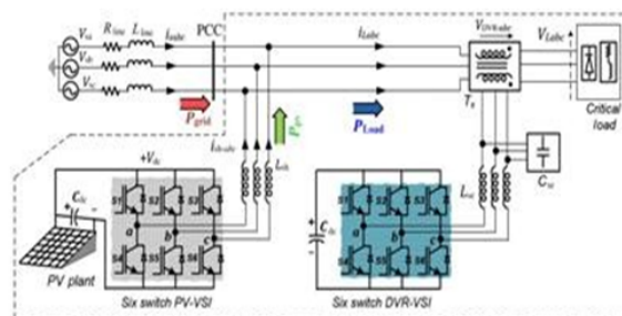
Fig. 1. On-site PV generation and sensitive load protection using self-supported DVR system.
