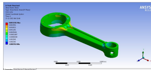
Figure 3: Maximum principal strain in connecting rod using AL 7075
