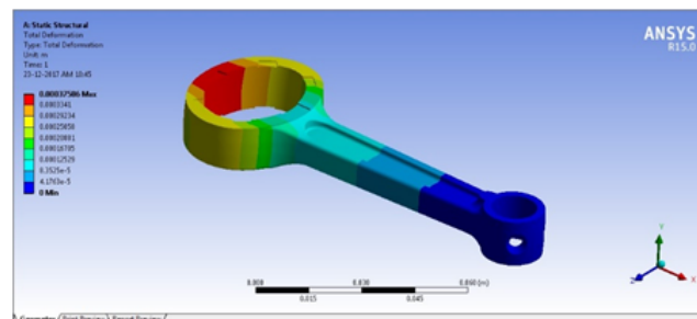
Figure 4: Total deformation in connecting rod using AL 7075
