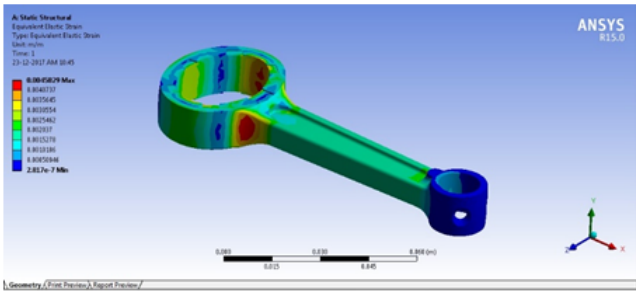
Figure 1: Elastic strain in connecting rod using AL 7075
