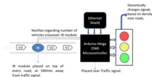
Fig 3.2.1: BLOCK DIAGRAM
