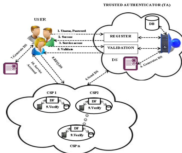
Fig. 2: Proposed Authentication Mechanism
