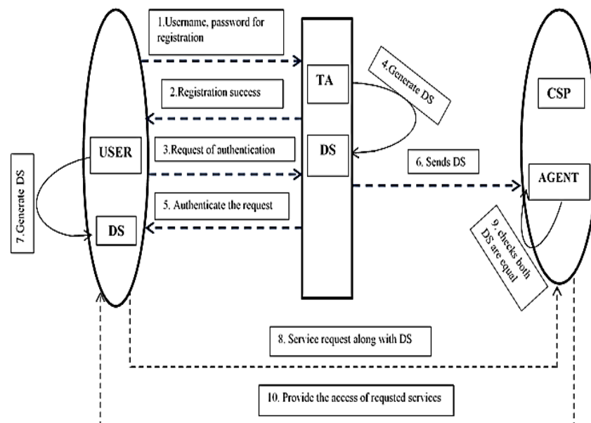
Fig. 3: Workflow of Authentication Mechanism
