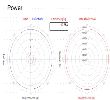
Fig. 5 Efficiency of fractal antenna in percentage
