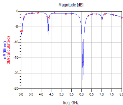
Fig. 3 S_{11} of fractal antenna between 3 to 8GHz
