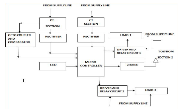
Fig 4 Schematic diagram of master section
