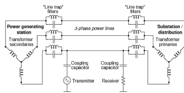
Fig 2 schematic diagram of existing system - 2
