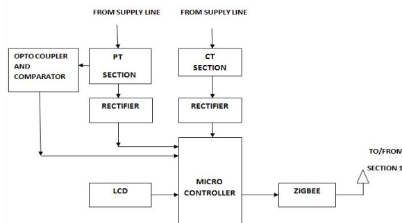
Fig 5 schematic diagram of slave section
