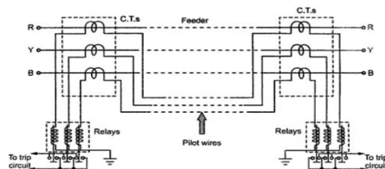
Fig 1 schematic diagram of existing system – i
