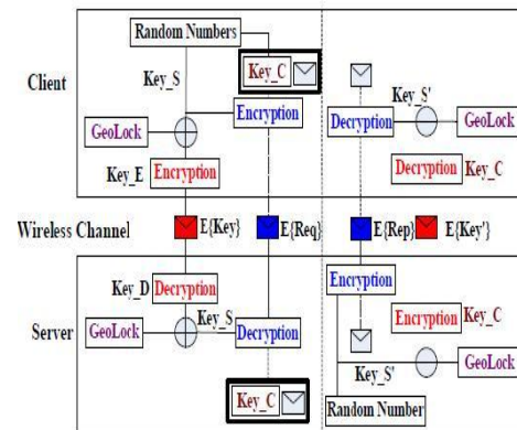
Fig 4. Illustration of Encryption and Decryption process.
