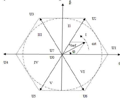
Figure (4) V_{ref} Mapped onto the Switching Pattern
