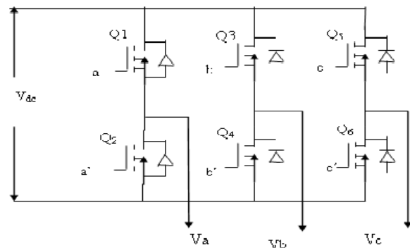
Figure (2) Basic Three Phase Voltage Source Inverter
