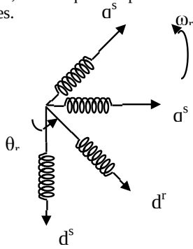
Figure 6: Equivalent two-phase machine for 3-phase machine
