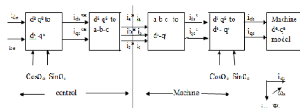
Figure(1) Vector control implementation principle with machine d^e-q^e model.
