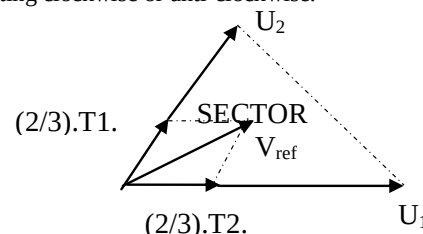
Figure (5) Generating V_{ref} in Sector 1
