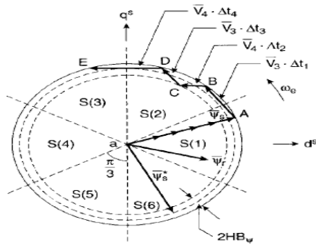
Figure (8) Trajectory of stator flux vector in DTC control
