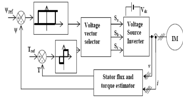
Figure (7)Block diagram of Direct torque & Flux control method.
