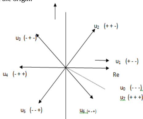
Figure (3) Switching Voltage Space Vectors
