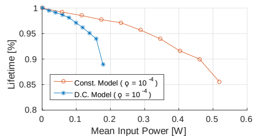
(b) Lifetimes for probabilistic harvesting, relative to constant harvesting
