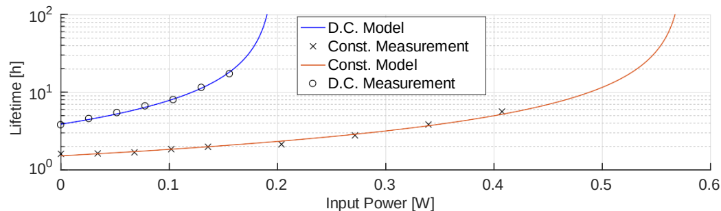
Figure 13: Measured lifetimes as a function of constant input power.
