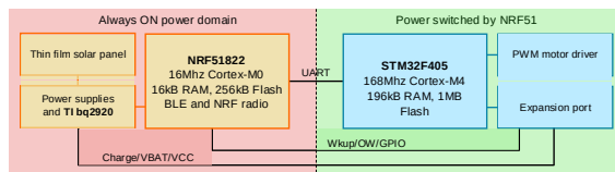
Figure 7: Crazyflie 2.0 electronics diagram.
