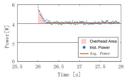
Figure 9: Power consumption of single rotor over two seconds @ 100% thrust.
