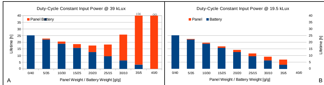
Figure 11: Weight distribution evaluation for constant input power. A - @ 39 kLux and B - @ 19.5 kLux
