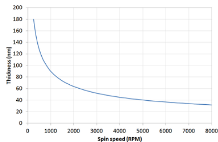
Figure 3. Thickness vs. speed graph
