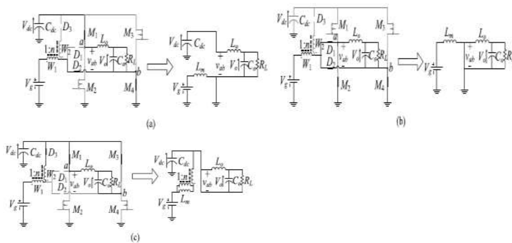
Fig.3. Topological states of the proposed SSBI and their equivalent circuits.
