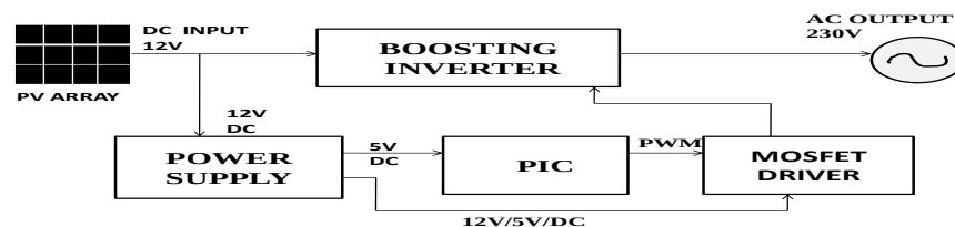
Fig.1. Block diagram of grid connected PV system
