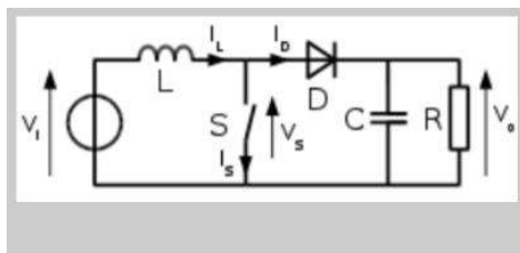
(Fig. 4. Boost converter schematic)
