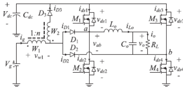
Fig. 2. Topology of the proposed SSBI.
