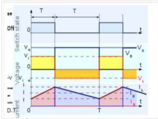
Fig. 5: Waveforms of current and voltage in a boost converter operating in continuous mode.
