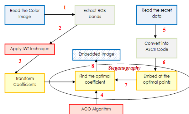
Fig. 2. Flow chart for the proposed algorithm
